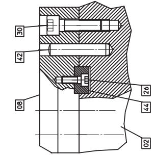
guide plate assembly 1:1
