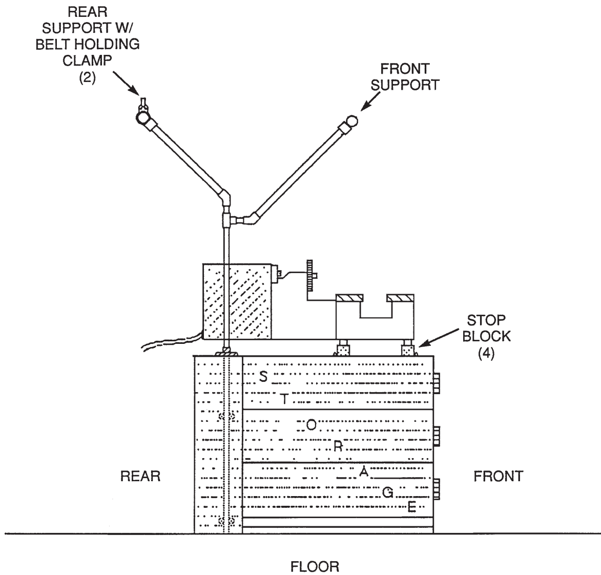
SIDE VIEW
