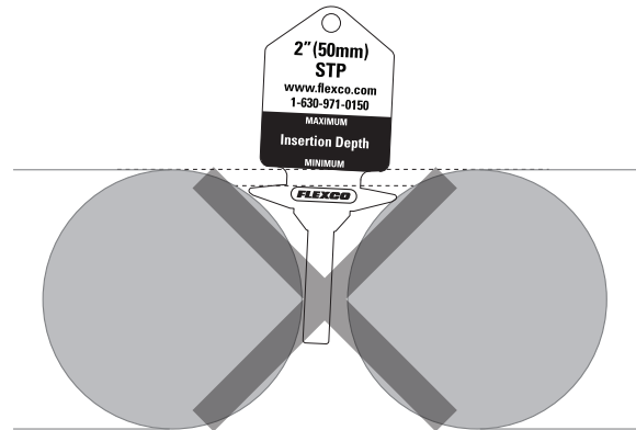
Misaligned between pulleys
