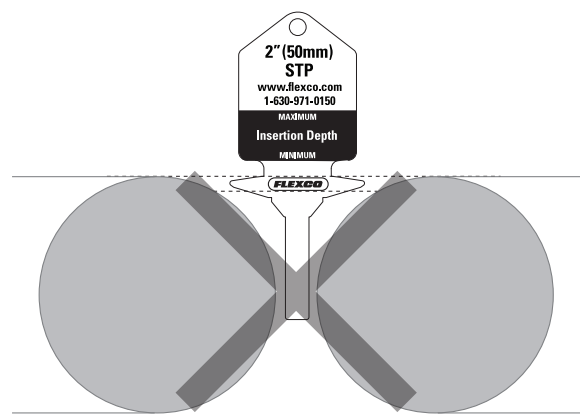
No contact with pulleys
