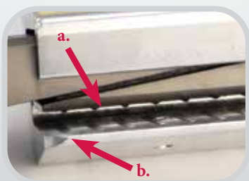
Ribbed lower wedge and grooved housing provide additional holding strength (a).
