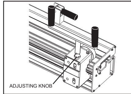
2. Position lacer head to the end of the tool. Turn knob clockwise to open rollers.
