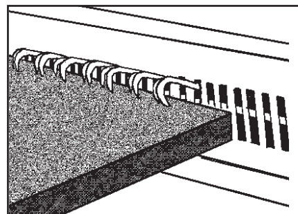
1. Guide belt through clamp; insert belt end into hook points and flush against the entire width of the face strip.
