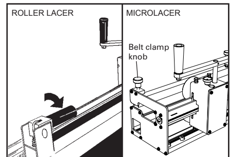
2. Lock belt clamp.
