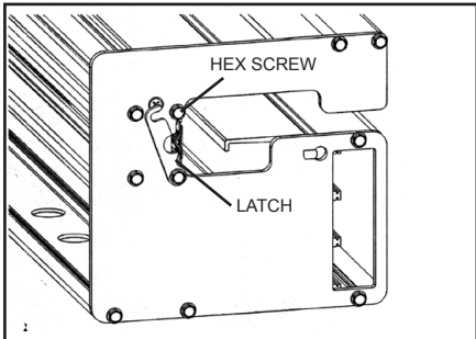
1. Loosen hex screw to allow Face Strip Retaining Latch to rotate out of the way. Insert Face Strip, reposition Latch and tighten screw.
