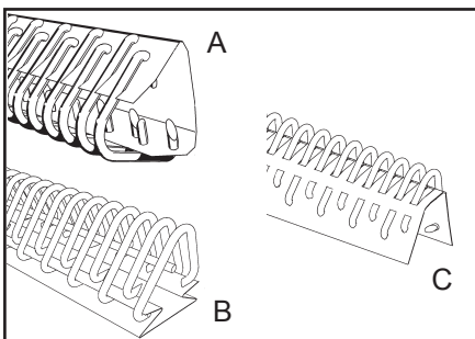
4. If using hooks as shown in A or B, remove carding paper at this time. If using hooks as shown in C, remove carding paper after installing hooks.
