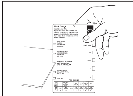
2. Select the proper size hook for your application.
