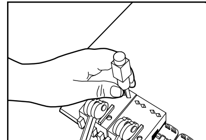
8. Very important — position staple driver in applicator and push staples down by hand until staples contact belt. Otherwise staples can wander when driven by hammer.
