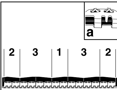
10. Follow the sequence shown above to drive all remaining fasteners. (a) Staples will be partially clinched.
