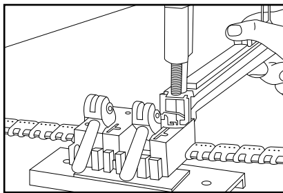
5. Use C150 staple dispenser for faster application. Position the staple dispenser over staple slots as shown. Push plunger all the way down by hand to insert staples.
