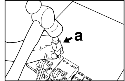
9. Starting with the center fastener plates, strike (a) staple driver with a 0.5 kg (1 lb.) hammer. Do not overdrive staples. Raise cam lever(s) to remove tool.
