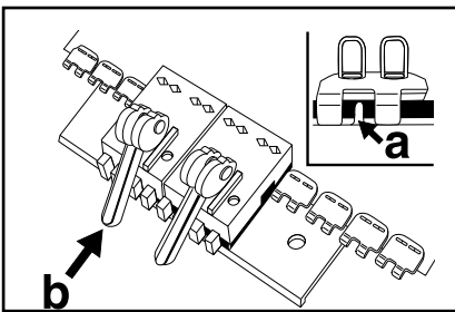
4. Belt end should be tight against the fastener (a) belt stops and fastener strip should be tight against the tool. (b) Depress cam lever(s).
