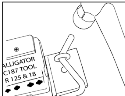
11. Tools 12" and over are furnished with a release bar which when tapped with a hammer releases belt from tool.
