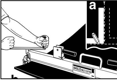
1. (a) Square belt using centerline method. Cut belt using using Clipper 845LD Belt Cutter or 900 Series Belt Cutter.
