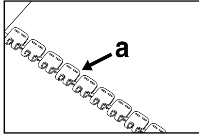
2. Place belt on solid surface for support. Center fastener strip, equal distance from the belt ends. (a) The word "Alligator" should be facing up.
