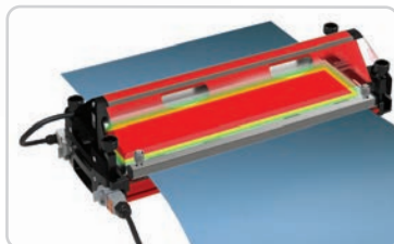
Wide Effective Heat Zone of 150 mm allows for easy positioning of the splice within the press.
