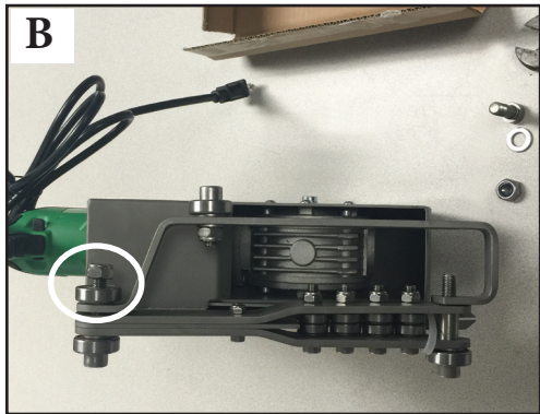
Step 3. (A) Remove bolt, washer, and lock nut from new retrofit rail kit. (B) Add washer, bearing, and lock nut to back of rail system.
