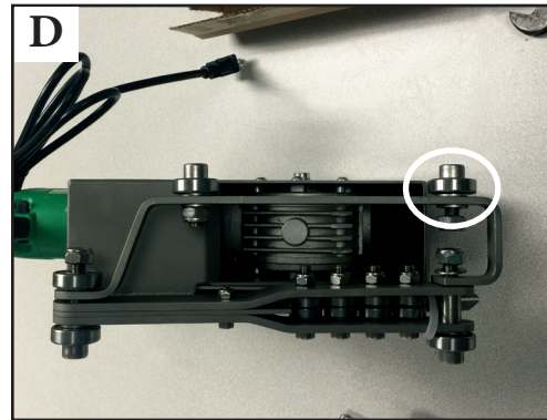
(C) Add washer and lock nut to front, center of rail system. (D) Add bolt, bearing, washer, and lock nut to front, outside of rail system.
