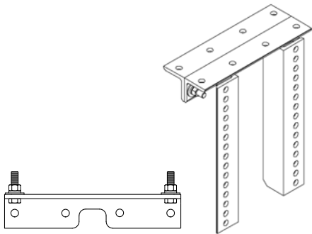
76073 SST Optional Top Angle Kit (for SST Tensioner) • Used with both standard and long mounting bracket kits for additional mounting options. • 13" (325mm) L
