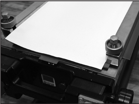
13. Place 0.5 mm silicone cloth (or silicone matrix pad) on top of prepared splice. Install Aero™ Press upper beam, attaching it to lower beam using connecting bolts.
