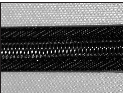
15. On the bottom side, belt inner-layer should melt, flowing slightly past belt ends, but not reaching spiral loops.
