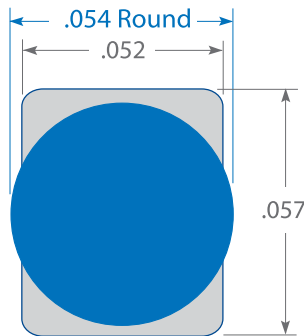
Cross-section of wire
