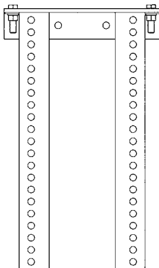
76072 SST Long Mounting Bracket Kit (for SST XD Tensioner) • For installations that require extra length legs. • 13" W x 21 1/2" L (325mm W x 538mm L)
