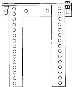
76071 SST Standard Mounting Bracket Kit (for SST XD Tensioner) • For most secondary cleaner installs. • 13" W x 15 1/2" L (325mm W x 388mm L)
