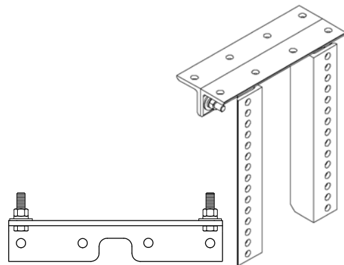
76073 SST Optional Top Angle Kit (for SST XD Tensioner) • Used with both standard and long mounting bracket kits for additional mounting options. • 13" (325mm) L
