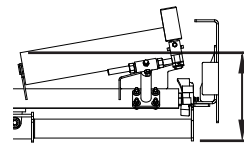
V-Return Clearance
