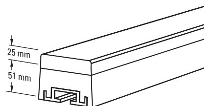
Impact Bar with 25 mm UHMW Cover
