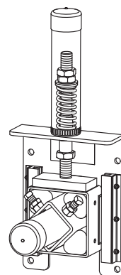
Spring cover on Secondary cleaner
