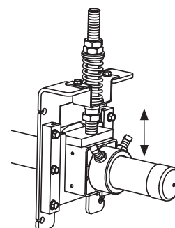
Secondary cleaner travel clearance
