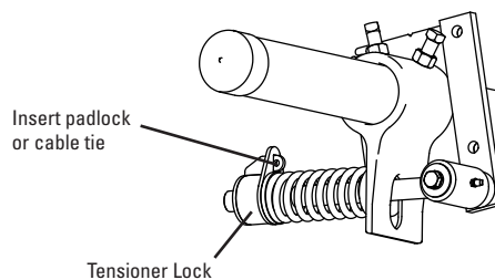
(Primary Cleaner tensioner shown)
