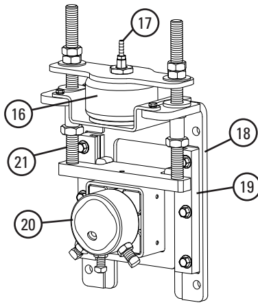
15 Secondary Air Tensioner XD
