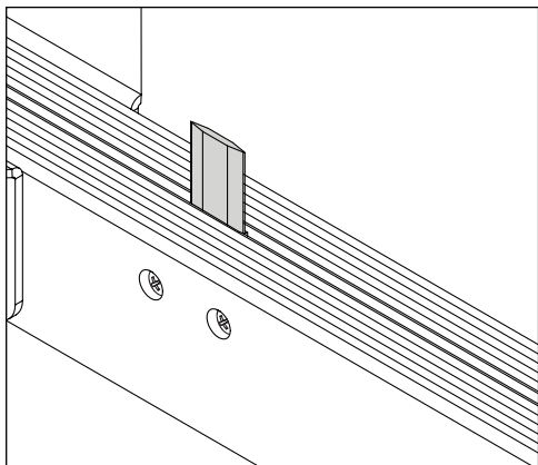
6. Tighten screws.
