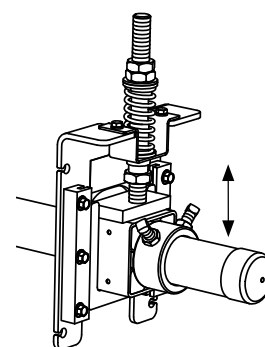
Secondary cleaner travel clearance
