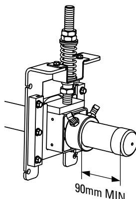
Pole length requirement outside tensioner
