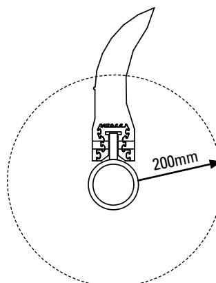
Precleaner 200mm clearance radius around pole
