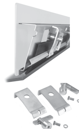
Bolt-On PAL PAK
