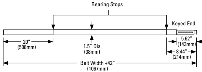
Shaft Measurements
