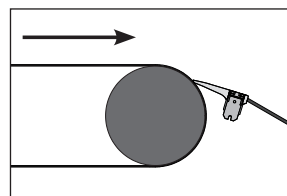
For belt to chute or slide applications. On pulley side, position no higher than 12 mm below the crown with bridge segment positioned roughly 3 to 12 mm above the top of the chute or slide back wall.
