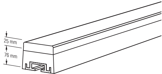
Impact Bar with 25 mm UHMW Cover
