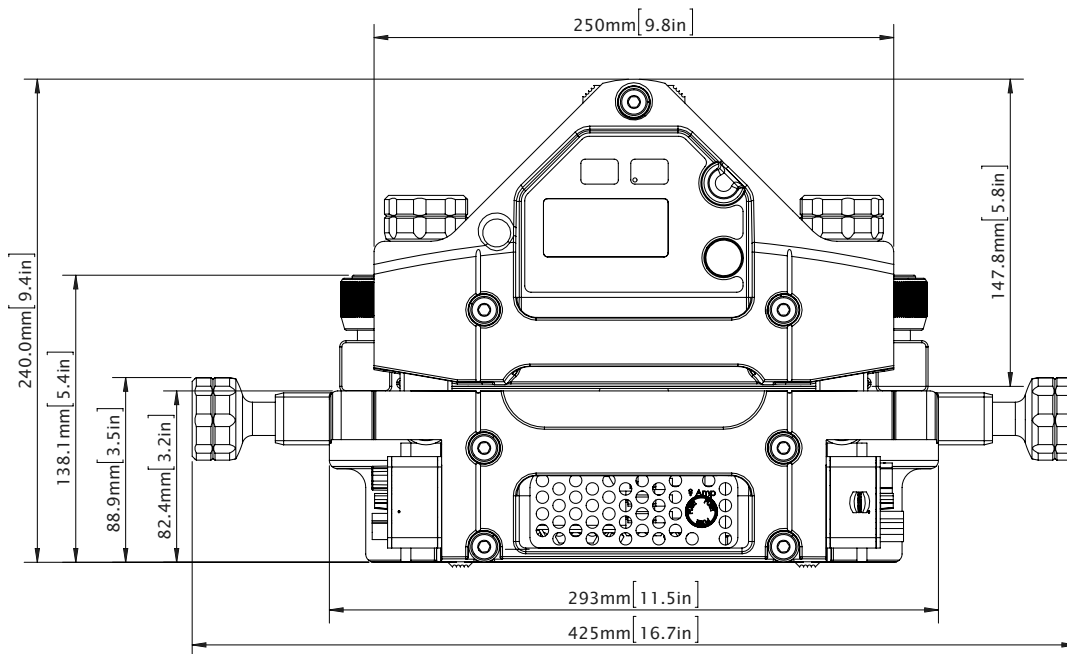
Front view and dimensions of Aero ® presses, sizes 625-1225.
