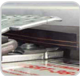
Riser plate allows for smooth transition of belt into fastener strips.
