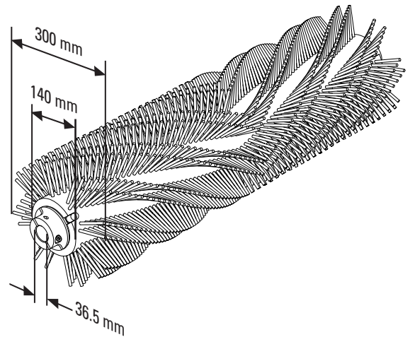
Shaft Measurements
