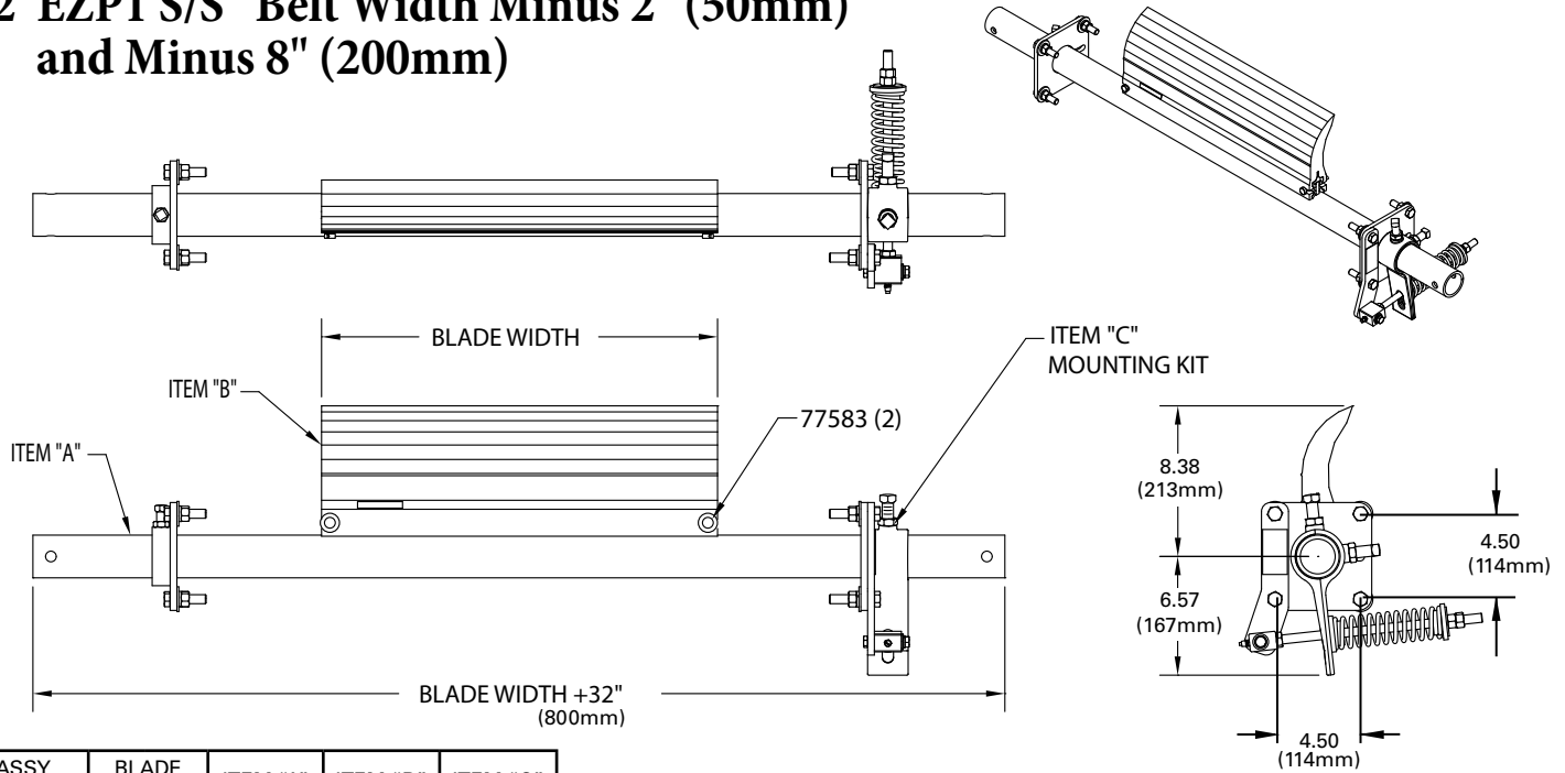
EZP1 S/S Belt Width -2" (50mm)
