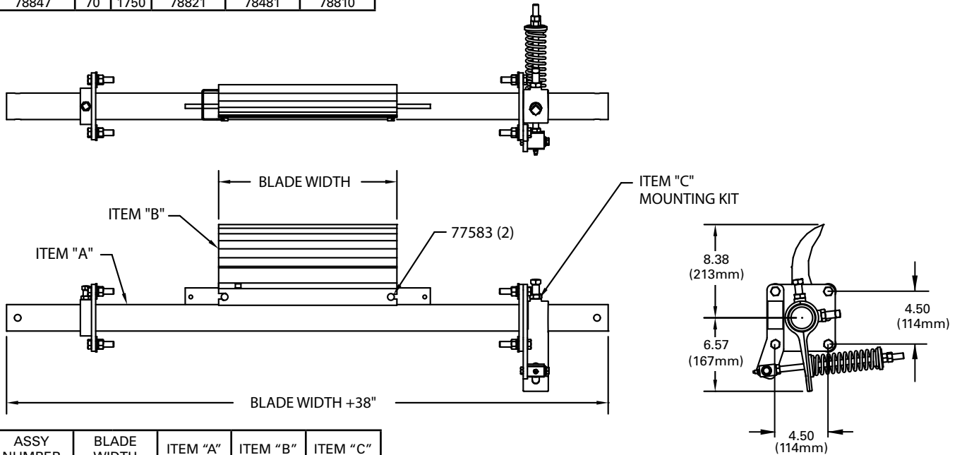
EZP1 S/S Belt Width -8" (200mm)
