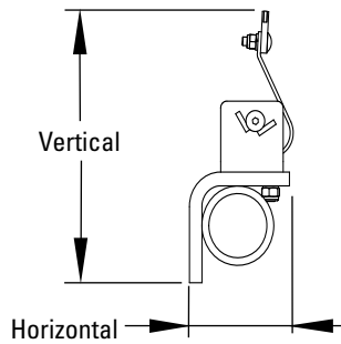
Clearance Requirement Specs
