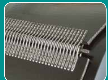
Flexco® Staple
