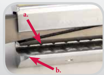
Ribbed lower wedge and grooved housing provide additional holding strength (a).
